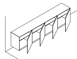
Wall-hung cabinet with doors to be fixed on wall, maxi weight: 109 kg/ml n.4 internal shelves
