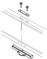
Two-ways joint and adjustable ground foot
