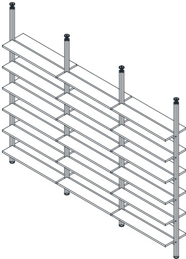
Double-sided bookshelf H. 270/300 cm with 6 shelves - 3 modules with 4 posts
