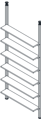
Single-sided bookshelf H. 270/300 cm with 6 shelves - 1 module with 2 posts
