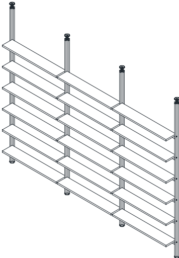
Single-sided bookshelf H. 270/300 cm with 6 shelves - 3 modules with 4 posts
