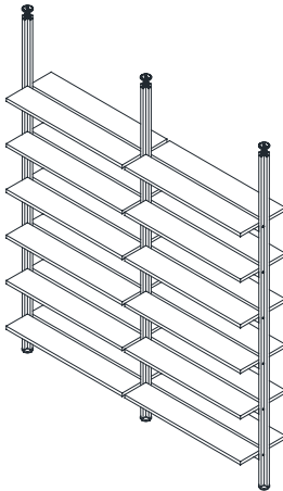
Double-sided bookshelf H. 270/300 cm with 6 shelves - 2 modules with 3 posts
