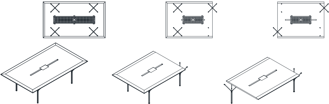
Rectangular tables with wooden top, shaped edge type A, central flip access door, cable tray, flexible cable riser with side zipper and 4-stem legs
