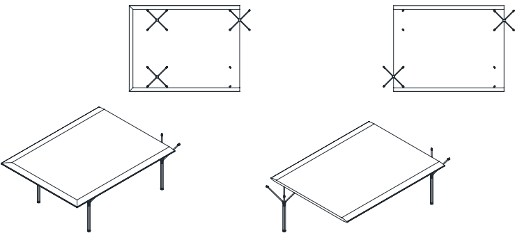
Rectangular terminal modules with wooden top, shaped edge type A and n. 3 legs with 4 stems
